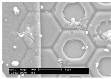
Fig 24. Sample image 4; after Al removal, close-up
