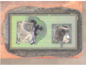
Fig 53. Sample image 61; 20 V, 3.5 A, 30 ms
