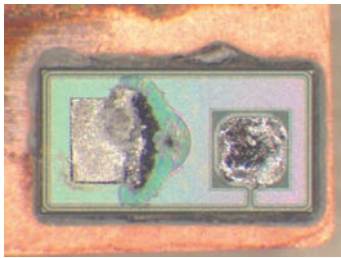
Fig 54. Sample image 62; 20 V, 3.5 A, 30 ms
