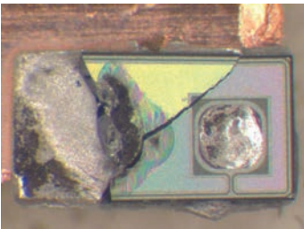
Fig 55. Sample image 63; 20 V, 3.5 A, 30 ms
